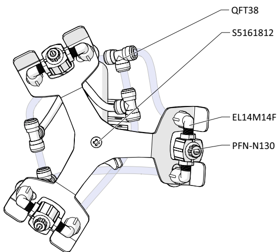
Fog Mast - Top View
